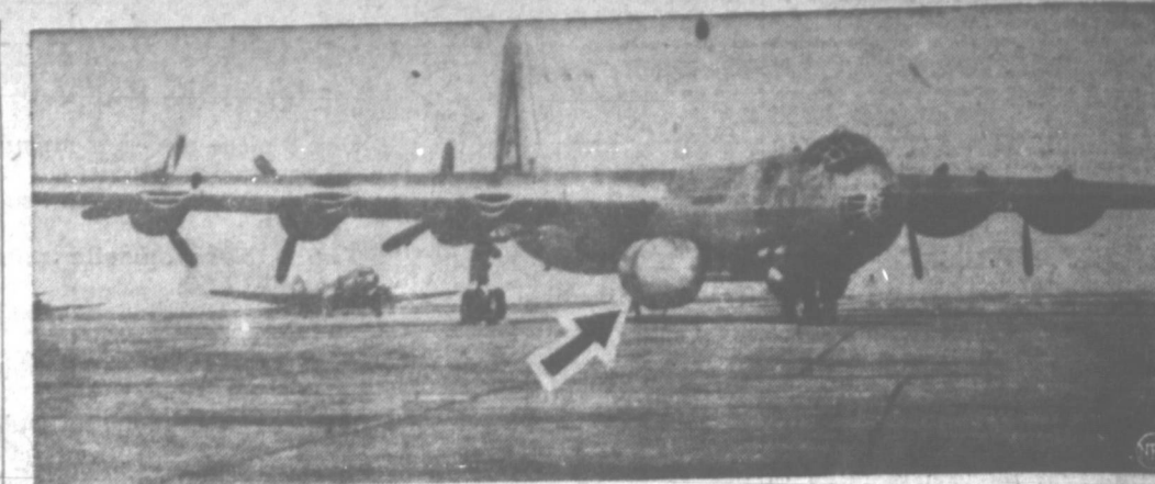
SUPERBOMBER CARRIES ITS OWN SPARES —Two complete spare engines, ready to install, are carried in nacelles (arrow) attached to the underside of the fuselage of this B-36-B Superbomber, seen at Fairfield-Suisun Air Force Base, Calif., after its first military test flight. Carrying spare engines makes the long-range bomber more self-sufficient when operating far from home base.
