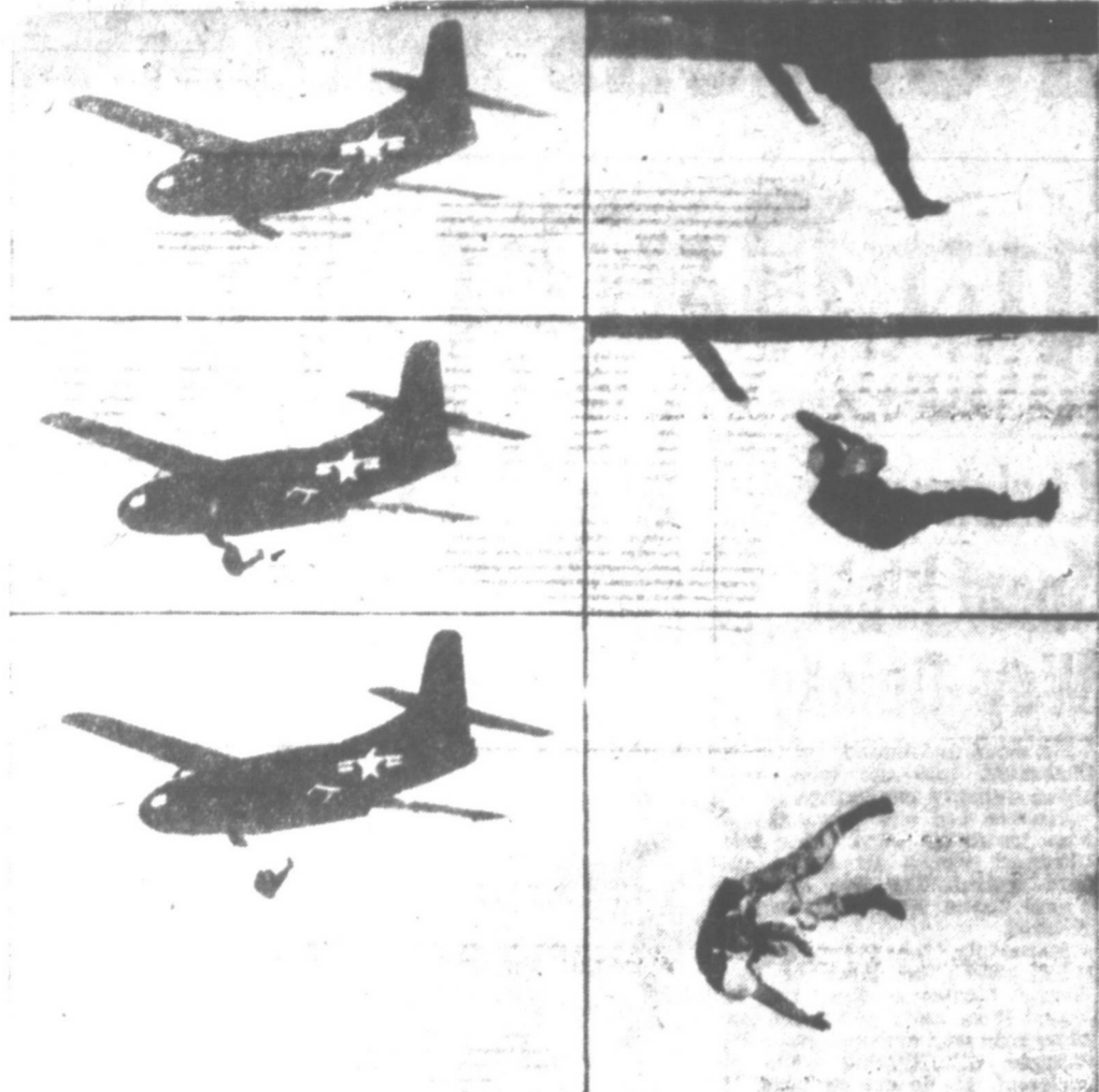
DOWN AND OUT —Unusual photographic sequence above shows demonstration of a new pilot ejection seat being tested on Navy F3D "Skyrider" jet fighters at El Centro, Calif. Conventional ejection device catapults the pilot straight up from his seat. In the F3D the pilot slides down a chute in the cockpit floor and drops out from the belly of the plane. Pictures, starting at upper left and going down, show pilot's course until he is completely free of ship and is ready to pull ripcord of his parachute. Successful "bailouts" of this type have been made at speeds up to 450 miles an hour.
