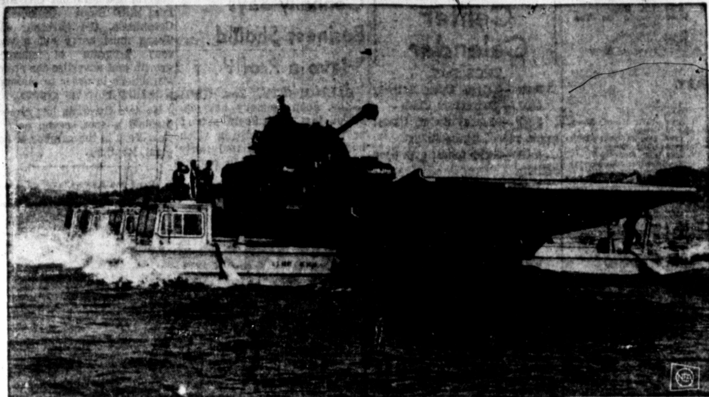
POTOMAC PASSAGE —A mobile floating assault ferry speeds a 47-ton tank across the Potomac River at over eight miles an hour. The ferry, designed at U.S. Army Engineer Research and Development Laboratories at Fort Belvoir, Va., is made up of four individual units, two of which carry ramps. On land, the units are disengaged from each other and travel at speeds up to 35 miles an hour.
