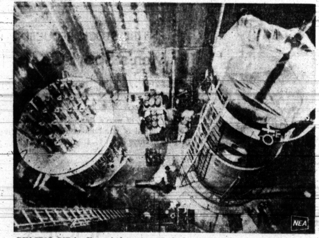
REACTOR PIT for Europe's largest pressurized water atomic power plant is seen under construction in Switzerland. It is due to be covered with its biological shield in early 1972 and, when completed, the station will have a capacity of five billion kilowatts.
