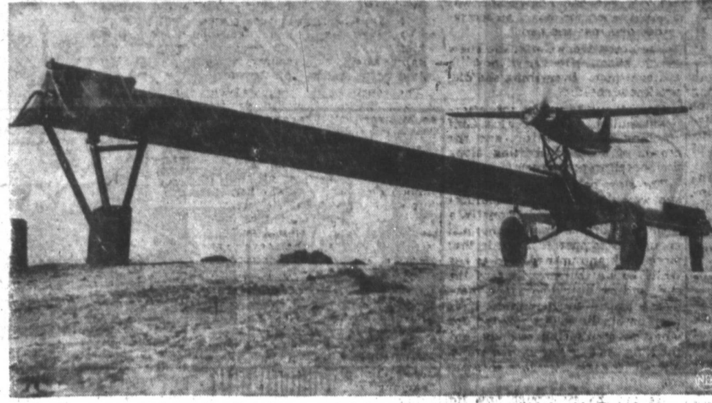
Taxiting along a 60-foot catapult, before a rocket launches it into the air, is the Air Force's new remote-controlled target plane, the OQ-19A. Shot into the air at a speed of 80 miles an hour, the tiny plane is capable of doing 220 miles an hour and performing intricate aerial maneuvers. The plane was tested at Wright-Patterson Air Force Base, Dayton, O.
