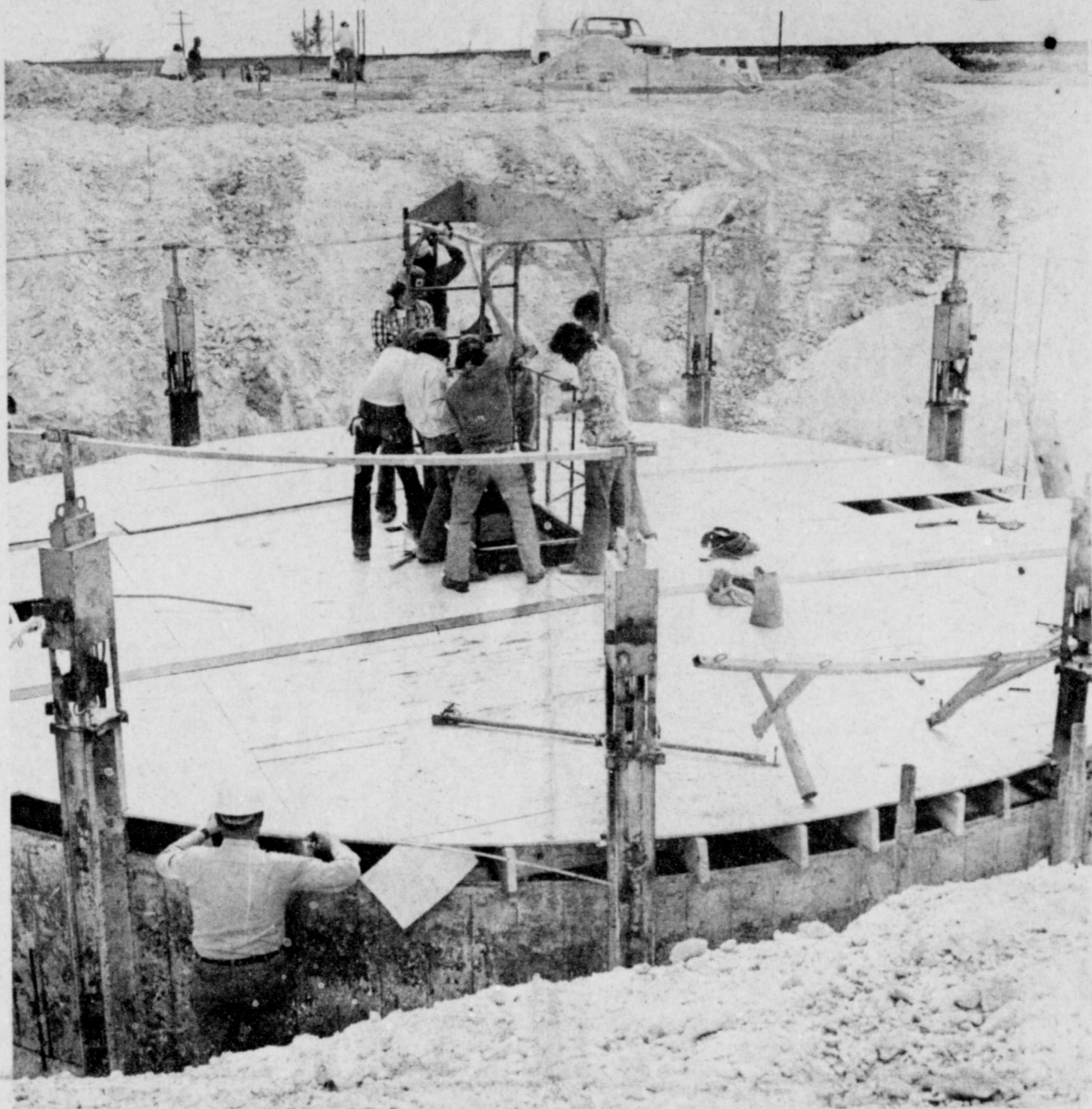
SILo WORK UNDERWAY--Valley Grain Products has construction underway at their location east of Muleshoe. Workmen here are preparing silo forms for the 25 silos being constructed at the site.
