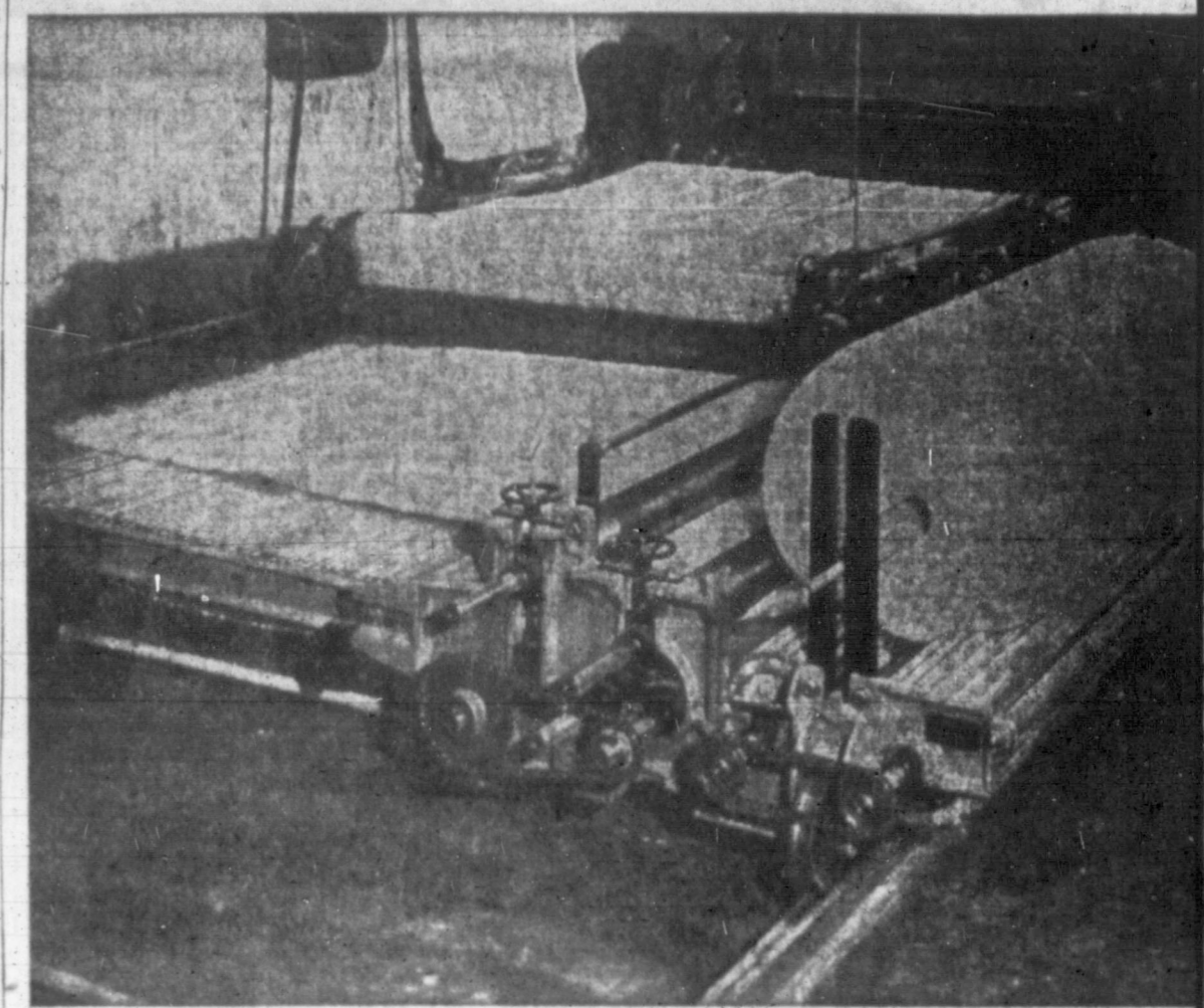
FELTING MACHINE — This is a complicated piece of equipment that lays the cotton in smooth quilted layers for a softer, more durable mattress. This is part of the factory type equipment at Acme Mattress Co., that is used to rebuild factory type mattresses.
