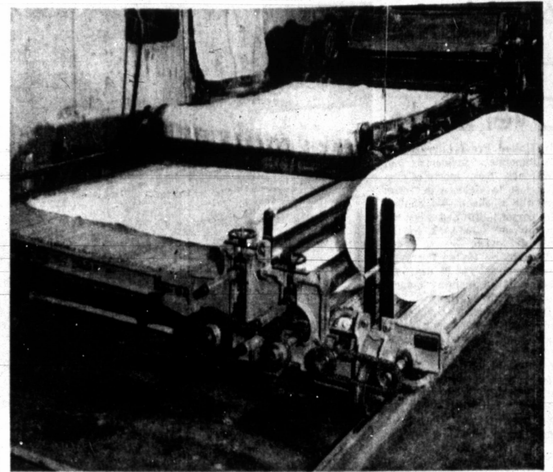
COMPLICATED MACHINERY — Pictured is the felting machine that is used in the construction of mattresses made at the Acme Mattress Co. at 817 W. Foster. This machine lays the cotton in smooth quilted layers for a softer and more durable mattress.
