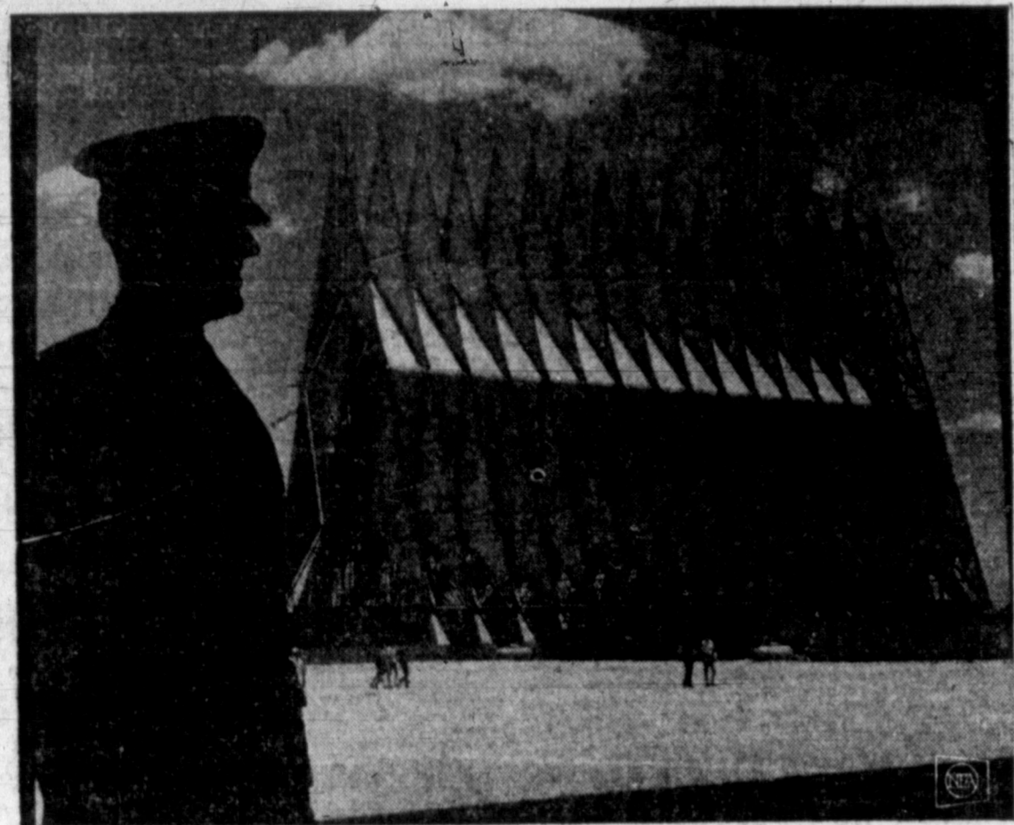
"THE CHURCH IS ONE FOUNDATION..."—A cadet is silhouetted against the modernistic interfaith chapel being built at the U.S. Air Force Academy at Colorado Springs, Colo. Constructed in triangular shapes of aluminum and glass, the 17-spire chapel will house a 900-seat Protestant chapel on the upper level and on the terrace a 500-seat Roman Catholic chapel and a 100-seat circular Jewish chapel.
