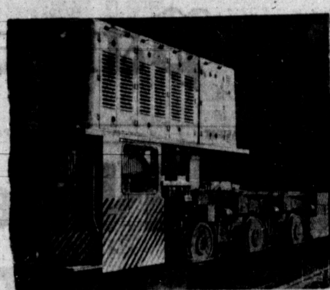
ODD ONE—A new look in locomotives. The motor's on top, engineer underneath. It's called a "side-arm pusher" and was designed for over-all visibility. It was built for pushing up to 50 cars at a coke plant in East Chicago, Ill.
