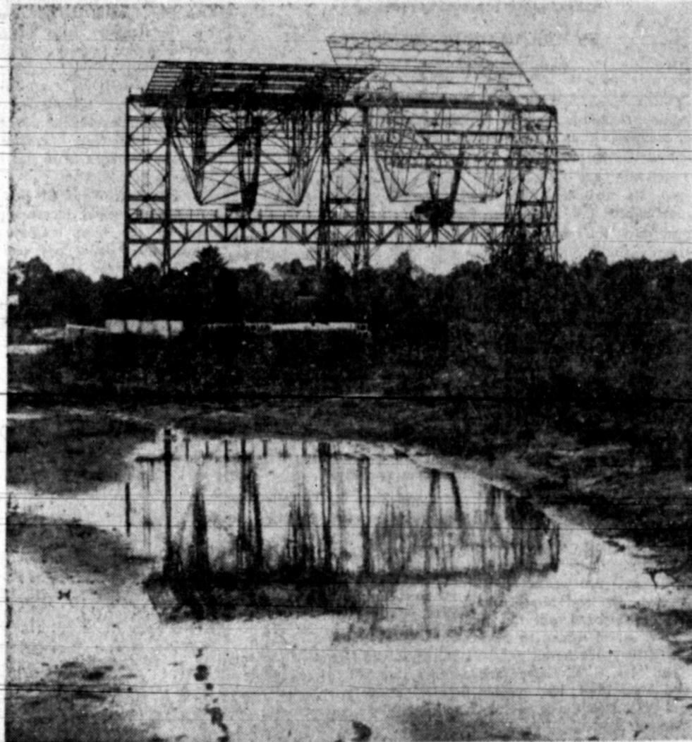
REFLECTIONS ON THE UNIVERSE —As it is mirrored in a nearby puddle, this huge apparatus is the antenna of a new radio telescope designed to listen in on the "universe" at Nancy, France. Moving on a horizontal axis, the antenna, 130 feet high and 250 feet across, will receive radio waves from distant galaxies in the cosmos.
