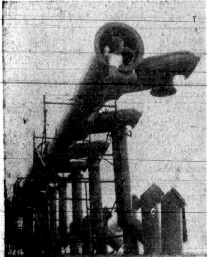
PIPING UP —In a tight squeeze, this workman goes inside what may be the world's largest single plastics installation, a 125-foot exhaust system. Newly completed in Evesville, Ohio, the system will be used to remove corrosive fumes from the zinc and tin plating lines of a steel plant. "A quarter-inch corrosion-resistant plastic sheet is used."
