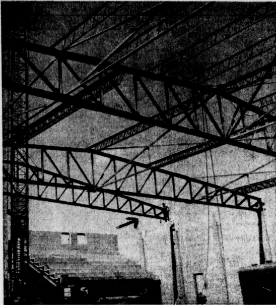
FINAL STEEL — Last truss in Muleshoe's elaborate building program was inched into place this past week as workmen lowered a 16,000-pound, 104-foot roof support into place at the new gymnasium (note arrow) with the aid of a 55-ton crane. (Journal Photo)
