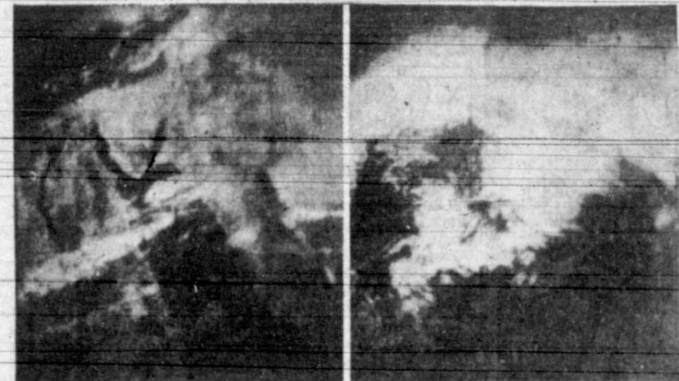
Photo, left, taken by Tiros' narrow-angle camera, shows Gulf of St. Lawrence looking west. Right: Sardinia, Corsica, Italy and clouds over the Alps are clearly visible in wide-angle shot.
