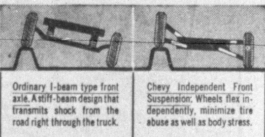
Ordinary 1-beam type front axle. A stiff-beam design that transmits shock from the road right through the truck.
