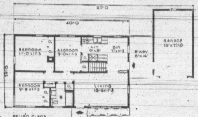
A SMALL HOUSE PLANNING BUREAU DESIGN NO. C-563
