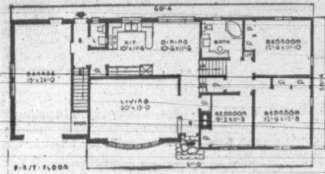
A SMALL HOUSE PLANNING BUREAU DESIGN NO. S-542
