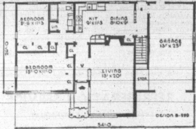
A SMALL HOUSE PLANNING BUREAU DESIGN NO. B-559
