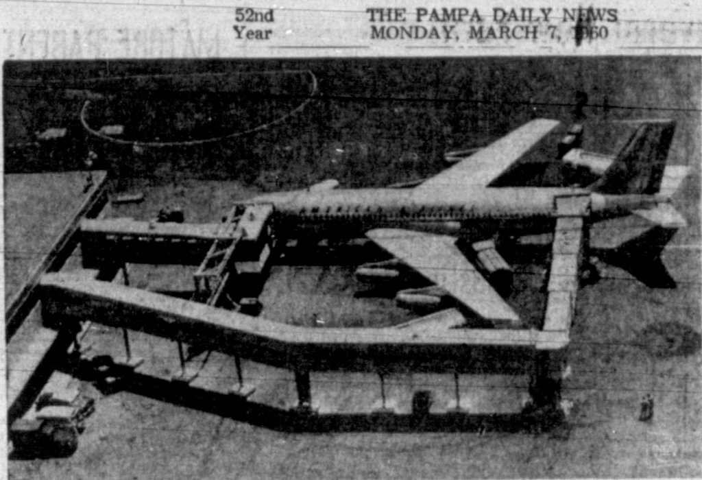
LOAD OR UNLOAD IN MINUTES—The minute this jet airliner braked to a stop at San Francisco International Airport, the two movable corridors of a "jetway" joined the fuselage at front and rear. The $100,000 unit can load or unload the 112-passenger ship in two to three minutes. The glass-enclosed, red-carpeted jetway protects the passengers from elements and airport fumes and noises. An operator controls the movements of the corridors from a panel.
