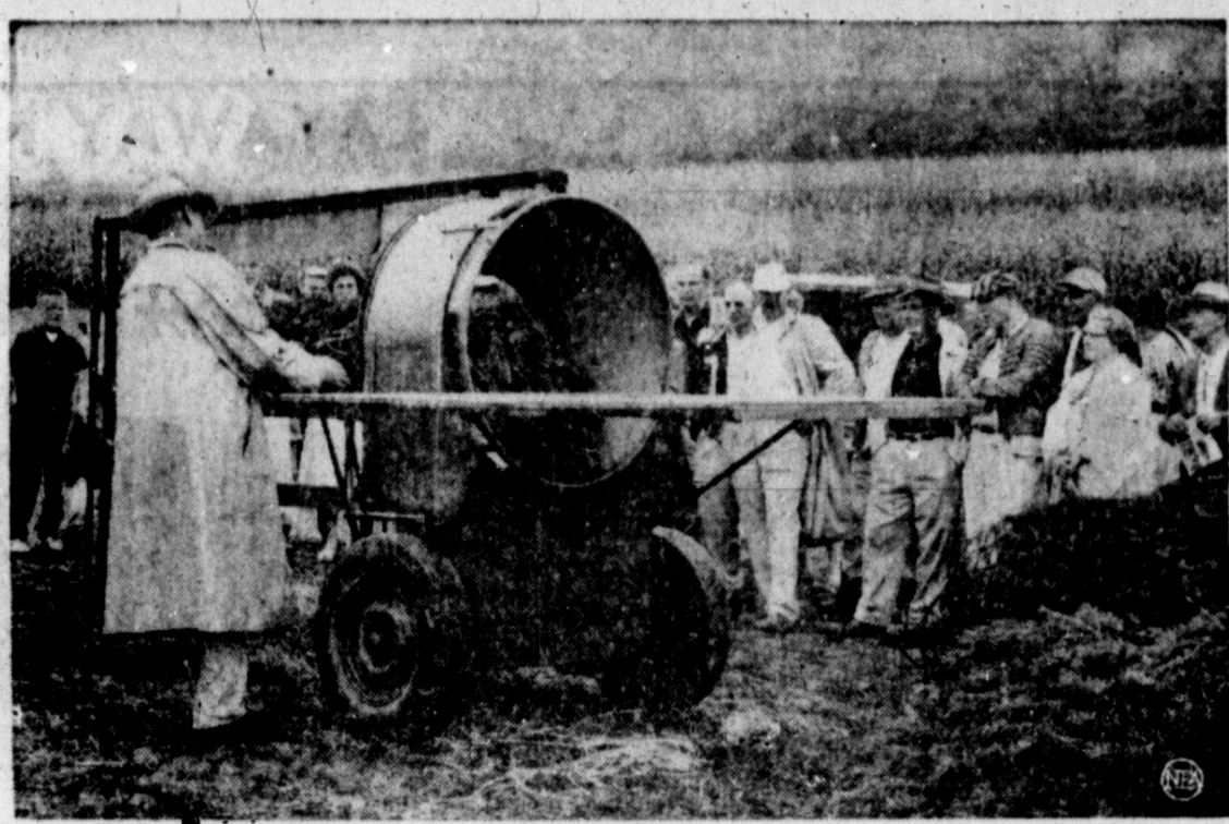
CHRISTMAS BUNDLES —One of the newest developments in the Christmas tree business is this wrapping machine. Handling from one to five trees depending on size, the machine bundles them neatly and binds the branches with cord for shipment to market. R. L. Larson of Smethport, Pa., demonstrates the wrapper.
