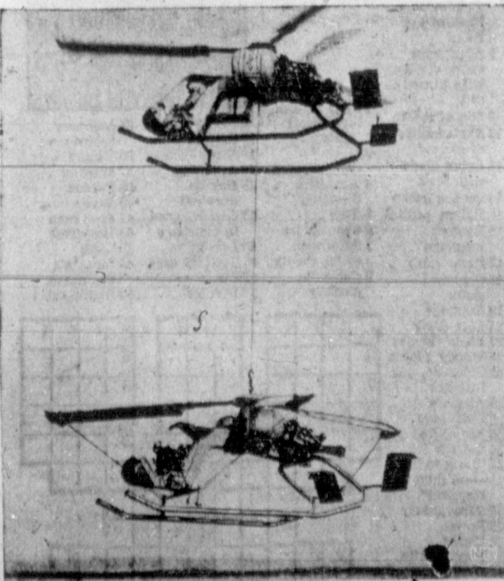
HEFTY HELICOPTER —Showing off its lifting capacity, one McDonnell Model 12 helicopter lifts another in a demonstration flight. It is powered by three gas turbine compressors. Compressed air is ducted to jets at the blade tips where fuel is injected and burned. This system eliminates power shaft, gear box, clutch and tail rotor. The copter has an empty weight of 2,400 pounds and maximum take-off weight of 8,300 pounds. Photo courtesy of Aviation Week.
