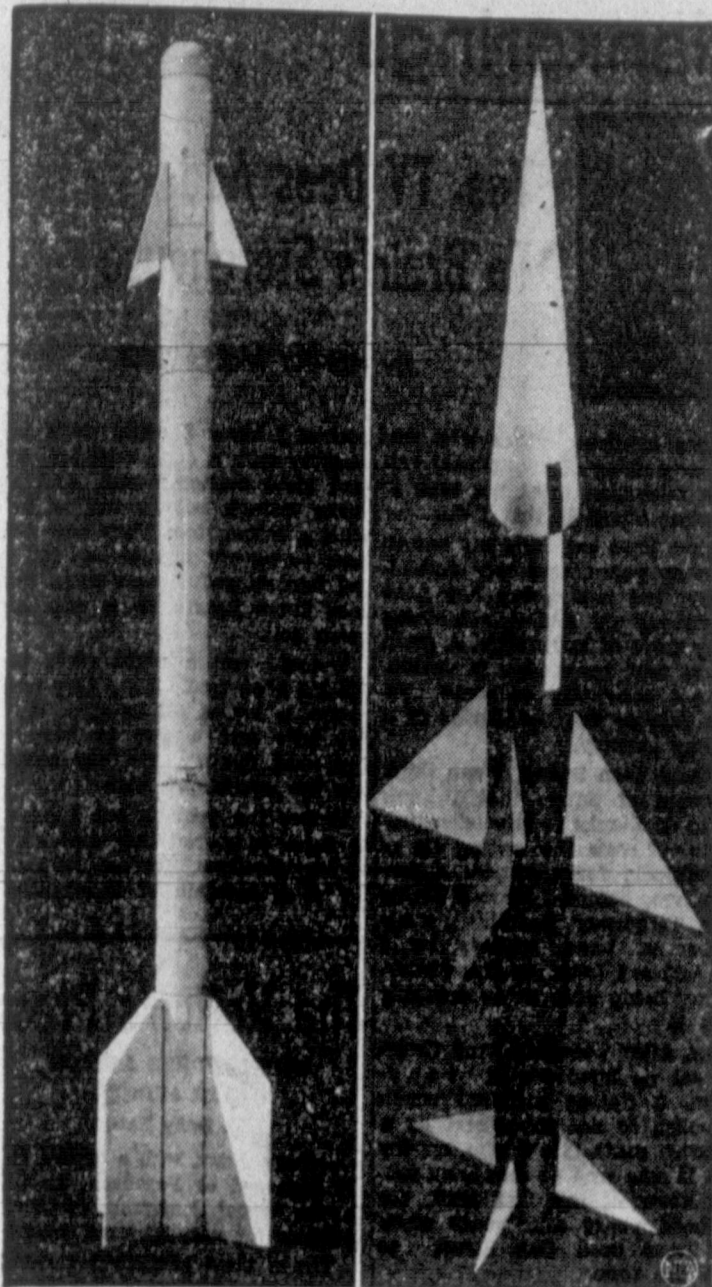
CHANGING AERIAL WARFARE —The Sidewinder air-to-air guided missile, left, met its first combat test with complete success. Chinese Nationalist pilots have been knocking down numerically superior Communist forces with the 1,200-m.p.h. missile which homes in on the enemy's jet exhaust by means of an infrared guidance system attracted to heat. It is 9 feet tall, 6 inches in diameter and weighs 165 pounds. About 300 m.p.h. faster is the newer radar-guided Sparrow, right, which has been assigned to U.S. carrier jets in the Formosan area. Sparrow is 12 feet long, 8 inches thick and weighs 350 pounds.
