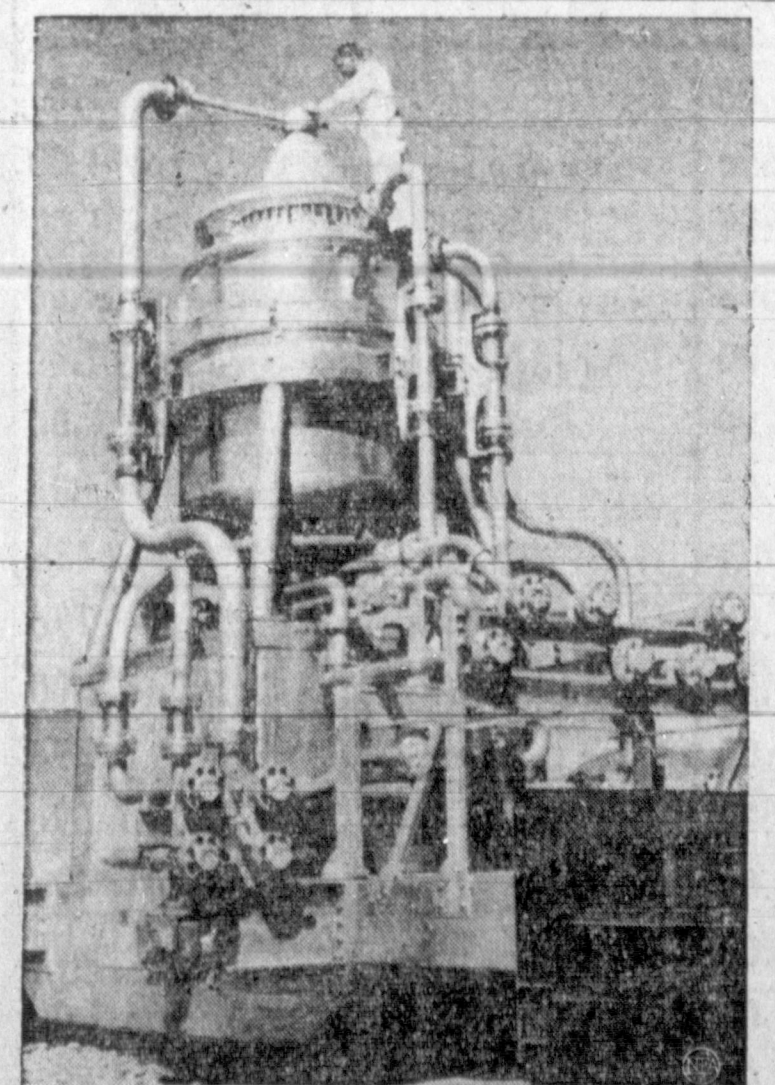
FIRST NUCLEAR ROCKET ENGINE —A prototype of what may be the rocket engine of the future is unveiled in Las Vegas, Nev. The Atomic Energy Commission, in projects Rover and Pluto, are testing the feasibility of nuclear propelled rocket and ram-jet engines. Charles D. Jakobiak of the Los Alamos Scientific Laboratory, examines the mockup of Kiwi-A, the first nuclear rocket engine which will be tested soon. The reactor is housed in the tubular structure below the nozzle. The entire unit is rolled into position on a remote-controlled railroad trolley.
