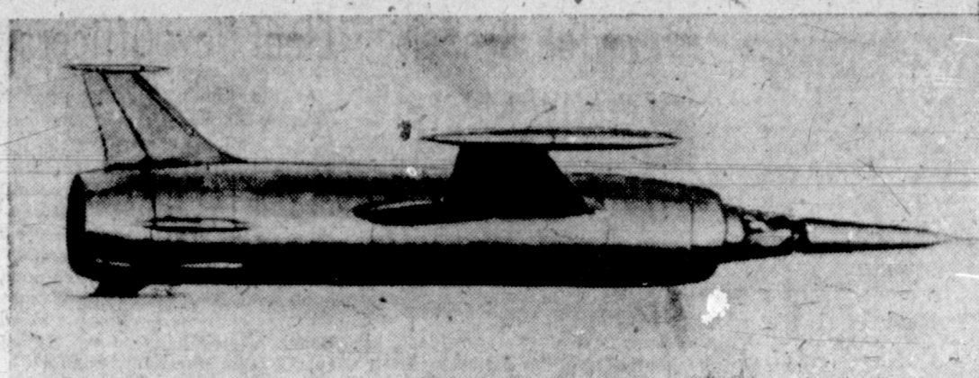
"FLYING STOVEPIPE"—This is the first photo released by the French Air Ministry showing the new supersonic Leduc 022, being tested at France's Istres airfield. The odd-looking aircraft, dubbed "The Flying Stovepipe" is powered by a ramjet engine that develops 600,000 horsepower. The eight-ton plane, made of heat-resistant alloys, is reported capable of flying at twice the speed of sound. The pilot flies in a prone position in its nose.
