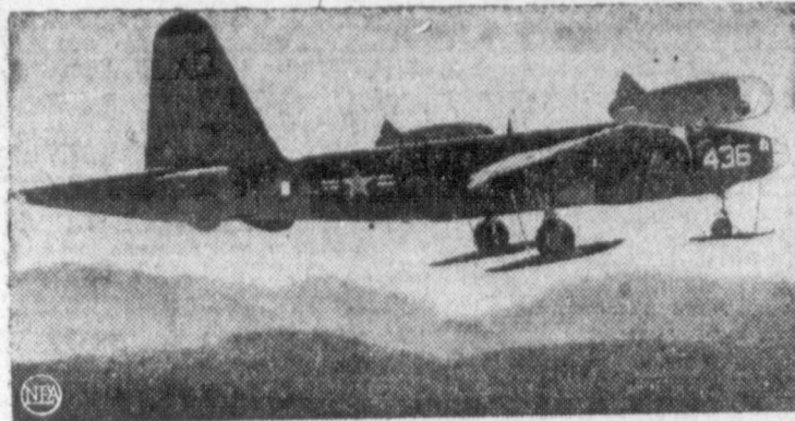
SKI JUMP —They don't look it, but those skis on this Navy P2V-7 Neptune over Ontario, Calif., are 16 feet long and five feet wide—the largest ever installed on a jet-powered plane. For takeoff and landing on dry land, the skis are retracted and wheels take over.
