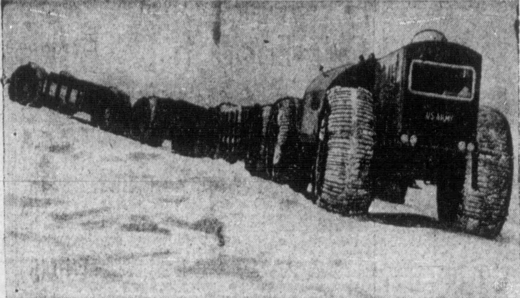
SNOW TRAVELING'S NO TROUBLE —A gigantic cross-country freight train, designed to tiptoe across deep snow fields, has been delivered to the Army Transportation Corps for use in the Arctic. The LeTourneau-built Sno-Train, above, rolls easily across three feet of snow during Army tests in northern Michigan. The tires stand 10 feet tall, and are four feet wide. Large "hubs" at the center of each wheel conceal powerful electric motors and gears which provide all-wheel drive. Built of aluminum, the Sno-Train carries 500 gallons of fuel, and comes equipped with a transparent bubble in the roof of the control car to aid navigation.
