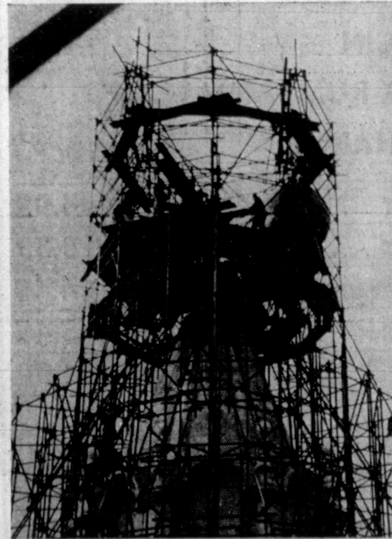
AFTER 300 YEARS —Workmen in Florence, Italy, are climbing over the cupola of the cathedral, which is encased in steel scaffolding, left. They were preparing to lower the giant cross-and-ball from its perch atop the 14th Century structure. At right, high above the city, other workmen attach the lifting gear. It was discovered that the great weight had weakened the cupola's top and there was danger of it crashing through the roof into the cathedral. This will be its first repair in 300 years.
