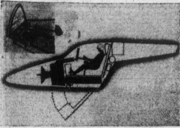
PARTING OF THE WAYS —A cockpit capsule which shoots off from the plane with its pilot, instruments and equipment inside has just been unveiled by the Navy. Developed by Douglas Aircraft, it was shown in model form at the recent Aeronautical Association meeting in Chicago. The capsule, forming the nose of the plane, is equipped with stabilizing fins, a "drag" parachute for use in the first stage of bail-out, and a main parachute system. Sketch shows how pilot sits in capsule and operates device that jettisons it. The capsule "may be ready" for use in 1958.
