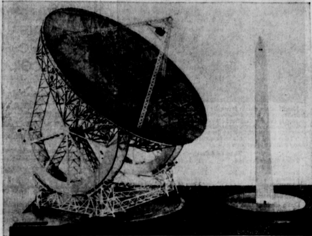
MONUMENTAL DISH SEARCHES SPACE—Scale replica of the Washington Monument is compared to a same-size model of the world's largest radio telescope. When completed at Sugar Grove, W.Va., it will reach out millions of miles into space searching for radio signals.
