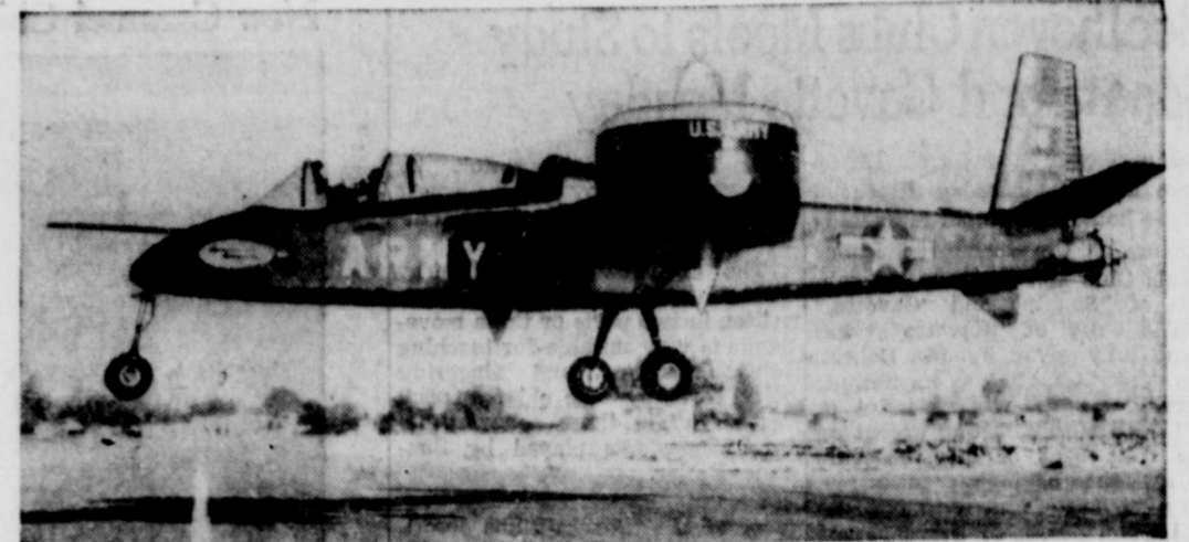
BARRELSFUL OF LIFT—Add to items in lift-by-the-bootstraps department the Army's Doak-16 VTOL (vertical takeoff and land) plane shown, above, at Torrance, Calif. The barrel-like gadget on the side of the plane contains the portside propeller. An identical unit is on the opposite side of the fuselage. In their present position, propellers lift the plane off the ground. Once altitude is gained, housings are rotated to face forward, and plane proceeds in horizontal flight.
