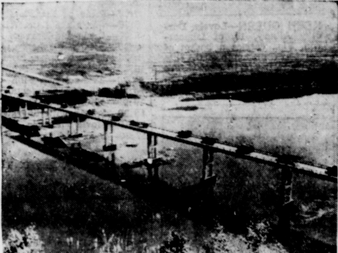
BUILT UNDER ENEMY FIRE, Libby Bridge spanning the Imjin River in Korea was completed by U.S. Army Engineers in five months, 21 days. The 1,074-foot span was named for the late Sergeant George D. Libby of Linden, N.J., winner of the Medal of Honor. The 84th Army Engineer Construction Battalion was awarded the Republic of Korea Presidential Unit Citation for building the bridge.
