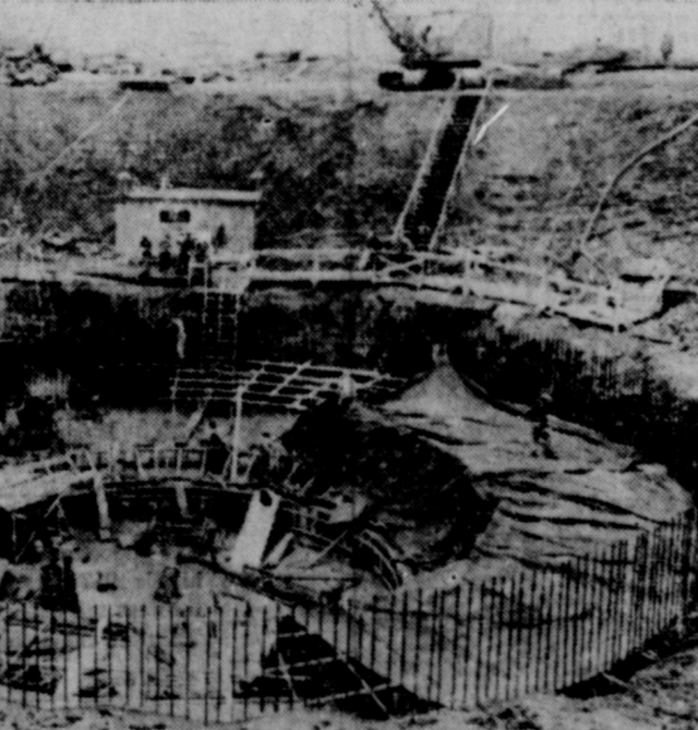
FIRST IN THE NATION—The first commercial-sized, breeder-reactor atomic power plant is gradually shaping up in Monroe, Mich. Shown is the foundation for the atomic reactor building, the dome-shaped unit which will provide the energy for the Enrico Fermi plant. Located at the bottom of a 56-foot excavation, the foundation itself is 20 feet deep and 87 feet across. The breeding process, scientists say, will extend the supply of atomic fuel to outlast the reserves of fossil fuels more than 50 times.
