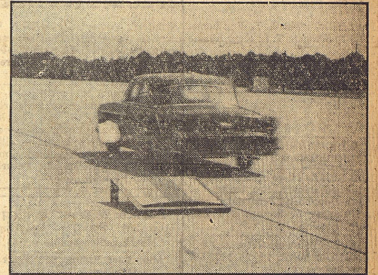
WHAM—Auto traveling at high speed slams 40-pound block of ice across section of fuselage of a C-130 Hercules turboprop troop and cargo carrier to determine effectiveness of various protective coatings.
