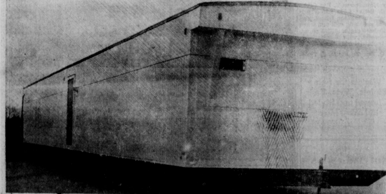
GIANT AZTEC rolls out—Largest mobile home built to date at Aztec Mobile Homes in Eastland is this enormous 14 by 70 foot model which rolled out of the plant recently. Bound for Louisiana, the model is significant to point out that Owner Larry Blalock and his crews can build on custom order or regular model to suit the customer. (Staff Photo)
