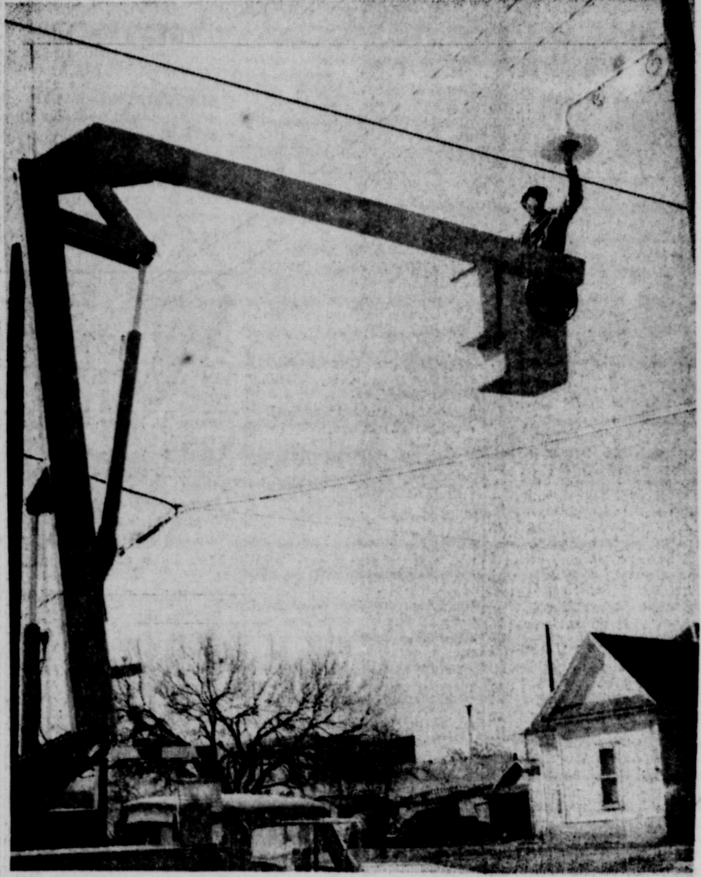
'SKY-HOOK'? — Texas Electric Service Co. employee Marlyn Jackson demonstrates the versatility of the company's new basket lift. It's sometimes called a "cherry-picker" or an "elbow left", but by any name it's proving to be a handy device for the linemen who are called on to go "upstairs" to repair lines and equipment. The basket itself is fiberglass, offering superior insulation protection for the operators who ride inside, with finger-tip control of the device. (TESCO Photo)
