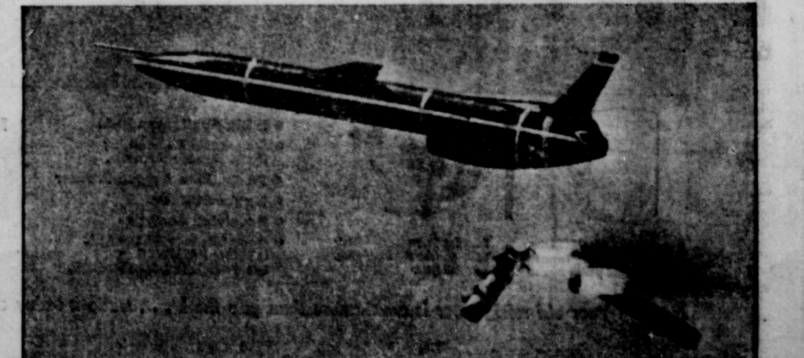
ON HER OWN—As flaming rocket boosters fall away, the Air Force's "Shark" noses along her over-water flight course after launching from Patrick Air Force Base, Fla. First of the nation's intercontinental ballistic missiles to be unveiled, the Shark is propelled by a turbojet engine. There's an automatic guidance system in the Northrop-developed missile which is designed to search out a target, day or night. It is unaffected by weather or temperature. In test runs, the nose carries electronic equipment which radiates performance data back to monitors. If launched during hostilities, the weapon would carry a warhead, presumably atomic in nature.
