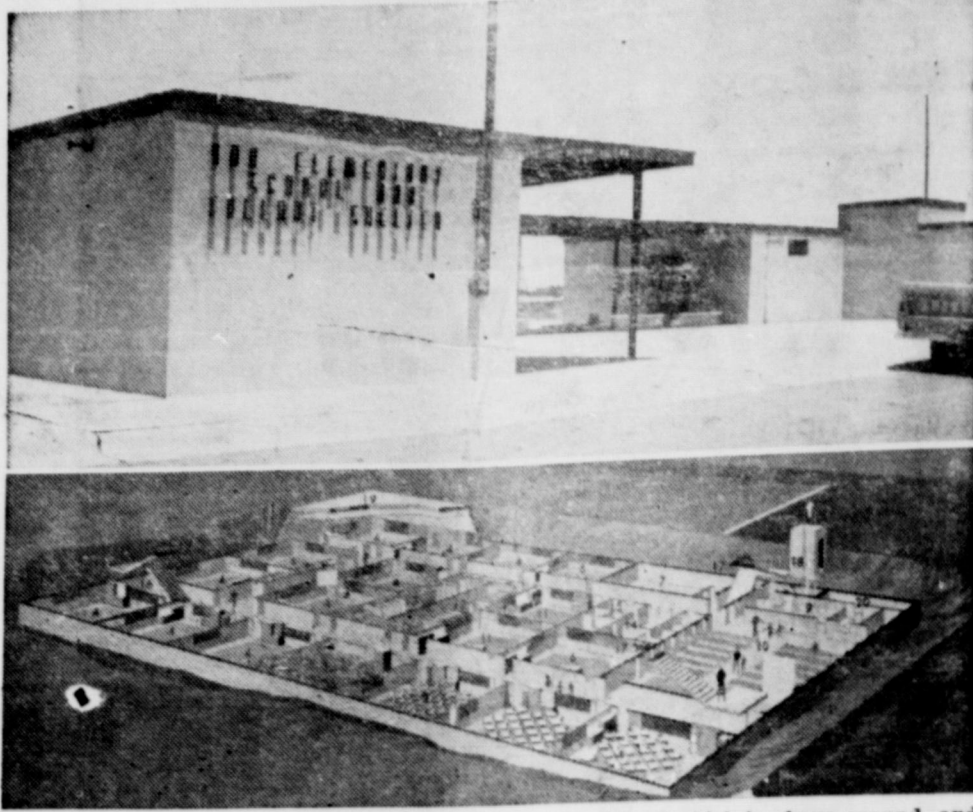
UNDERGROUND SCHOOL recently dedicated at Artesia, N.M., is an example of how functional construction can be combined with community fallout protection. Shown is the small portion of the $470,000 Abo Elementary School which is above ground, and a cross-sectional sketch of the underground facilities and supplies for 545 students or 2,000 shelter occupants. The underground school is the first of its kind in this country.
