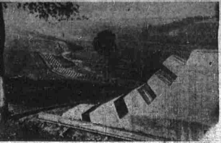
Spiked concrete barriers to trap invading tanks; part of the defenses protecting the Limes line.
