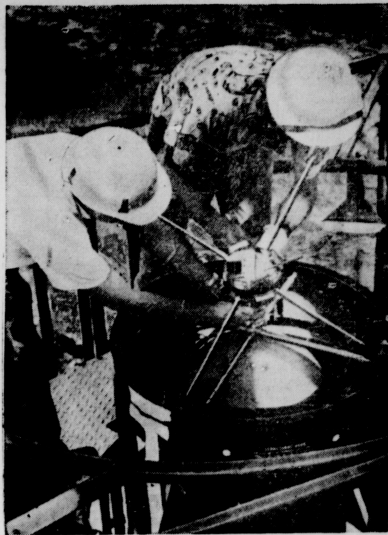
FIRST U.S. MOON INSTALLED —Engineers carefully install a 6.4-inch, 3¼-pound baby satellite at Cape Canaveral, Fla., launching site of the Vanguard rocket. The small satellite is fitted atop the third stage of the rocket, later to be covered with a nose cone. The aluminum sphere is a substitute for the 20-inch, fully instrumented satellite which will be launched when rocket tests are completed.
