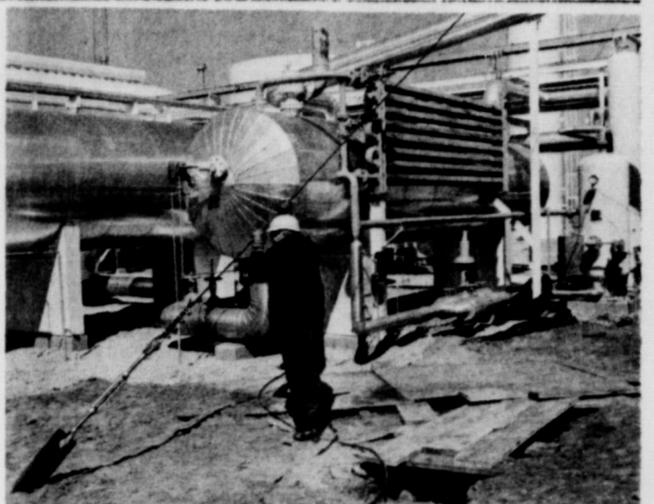
WORK BEGINS: Work begins on the expansion of facilities at Natural Gas Pipeline Company of America's Buffalo Wallow gas treatment plant. Ed Wright (pictured above) is Pipeline Supervisor for the local plant.
