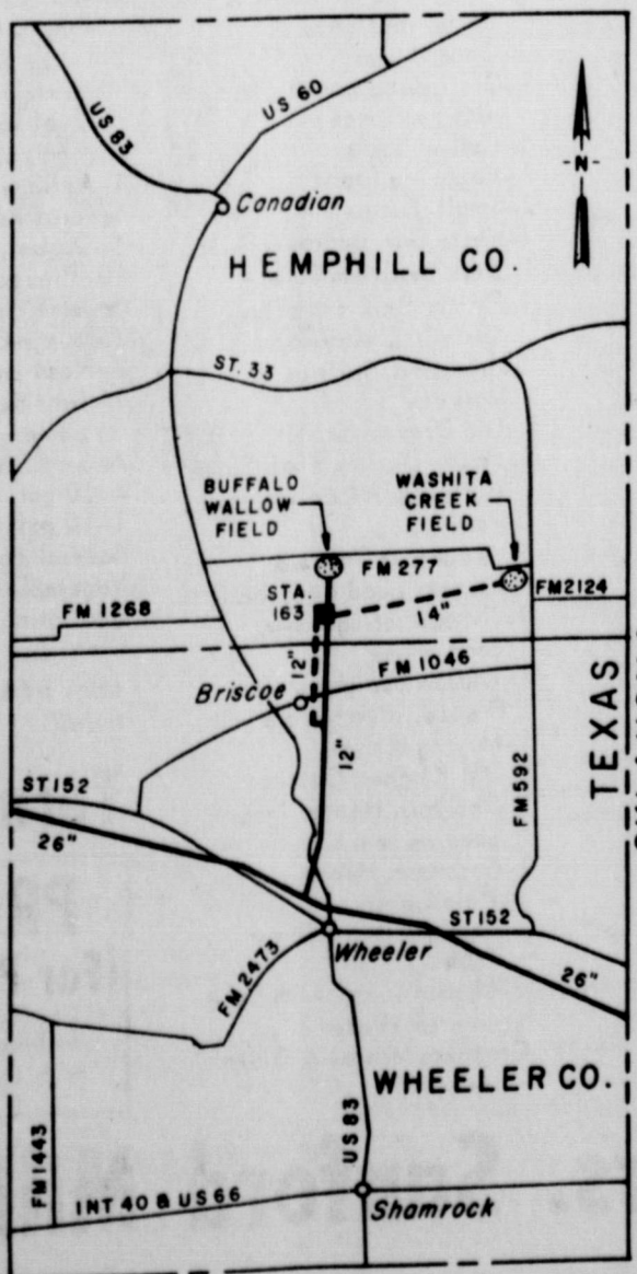
NEW LINE: Dotted lines indicate new facilities proposed by Natural Gas Pipeline Company of America in Hemphill and Wheeler County, Texas. An addition will be added to purification plant in Hemphill County.
