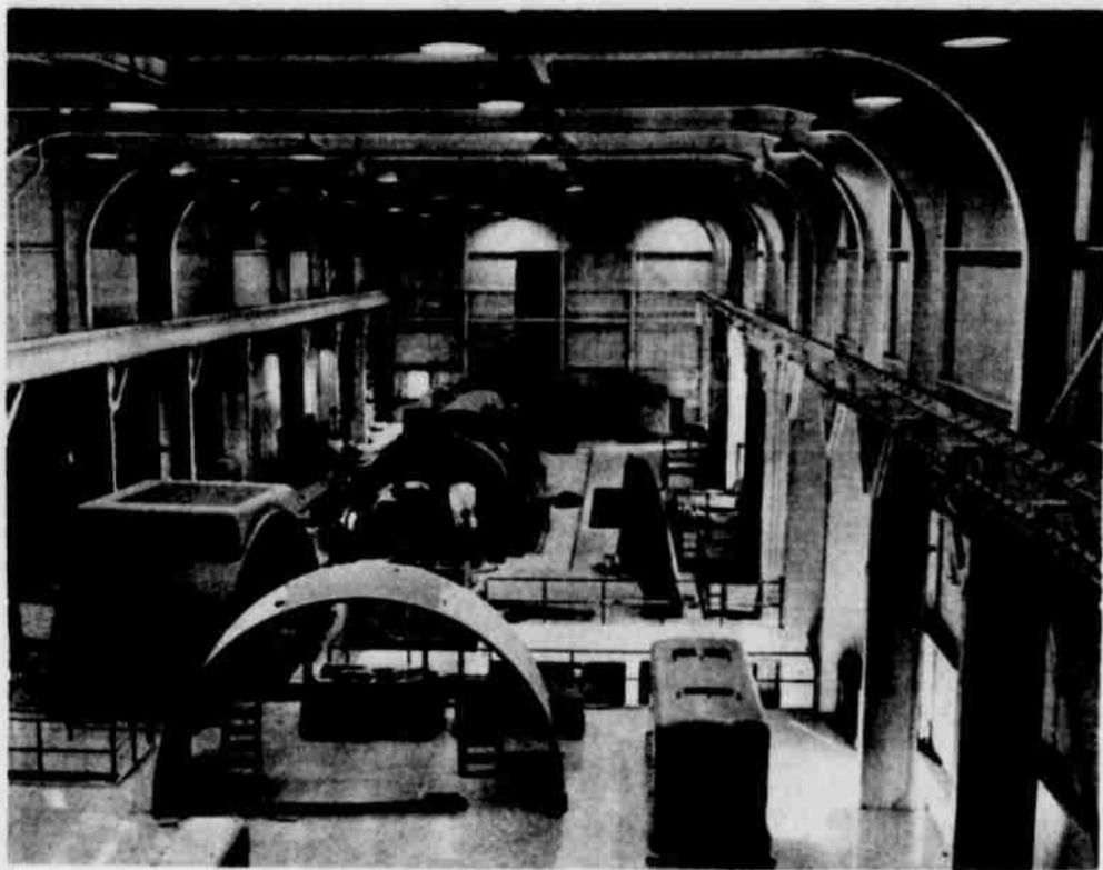
UNDER CONSTRUCTION at Southwestern Public Service Company's Plant X in Lamb County is a 210,000 kilowatt generator. The largest unit ever installed on the company's system, the huge turbo-generator will go into
