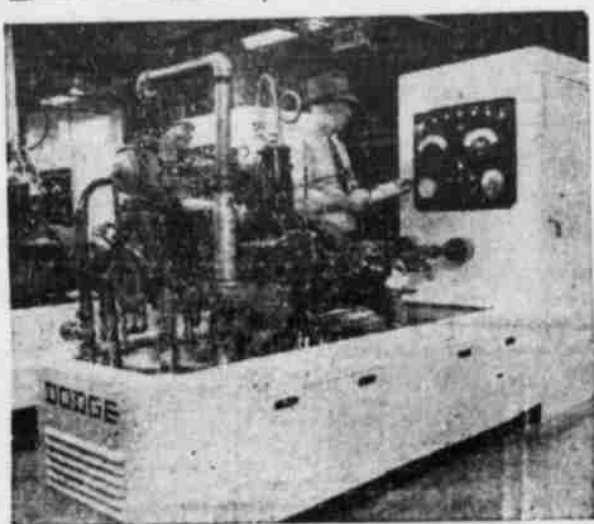
Car engine testing has become a precision operation, completely automatic and electronically controlled. This new dynamometer room is one of the showplaces of the Dodge Main Plant in Detroit. Engines on test generate 510 kilowatts of the plant's electric power per hour—without coal.
