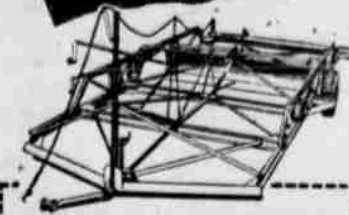
MODEL 25 - Width 12'10", length 33', cutting blade length 9'3", depth 23", requiring 38 H.P. (drawbar).
