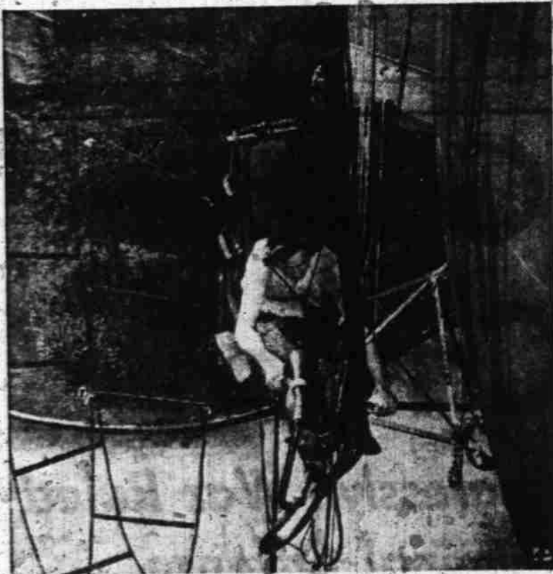
ATOM SMASHER TESTED — An X-ray technician tests the soundness of welded seams of a electrostatic generator at the Westinghouse laboratories, Pittsburg, Pa., as the atom-smasher is readied for research into nuclear physics. His telephone headset enables him to talk to another technician who co-ordinates operations with those of a film-handler inside tank.
