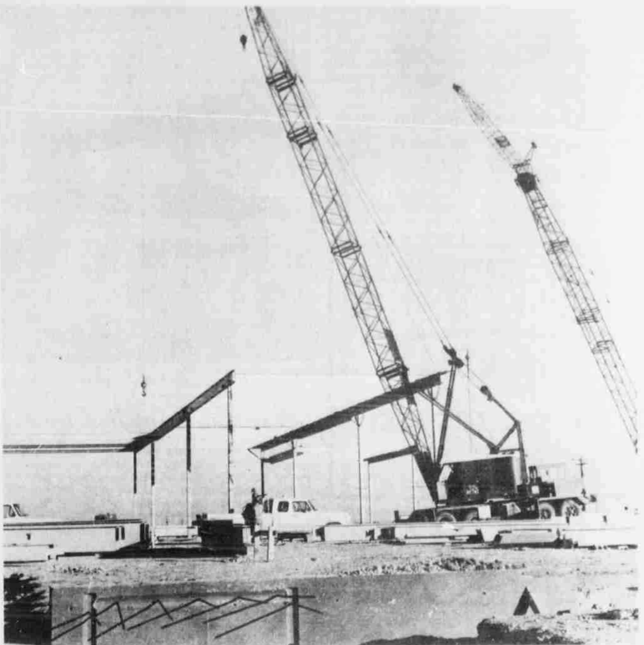
STEEL ERECTION got back underway by Wednesday of this week at the American Cotton Growers Denim Plant despite wind damage totaling from $10,000 to $25,000 during the storm last Saturday. Bob Hale said steel erection had just started Friday before the Saturday storm. The high winds blew some uprights over, twisted some, damaged flanges and connecting
