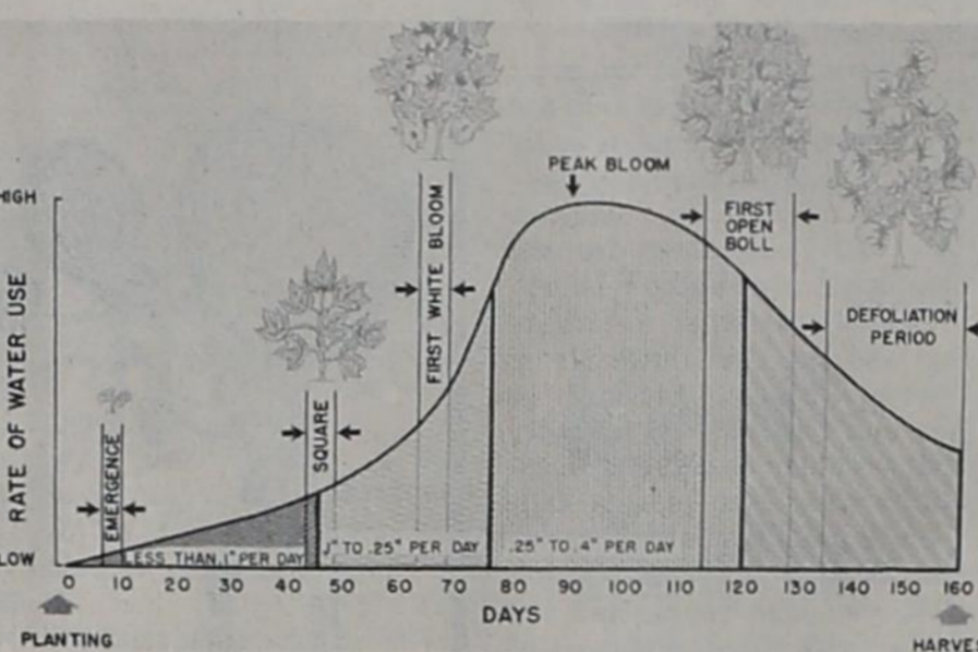
Daily rate of water use by cotton.
