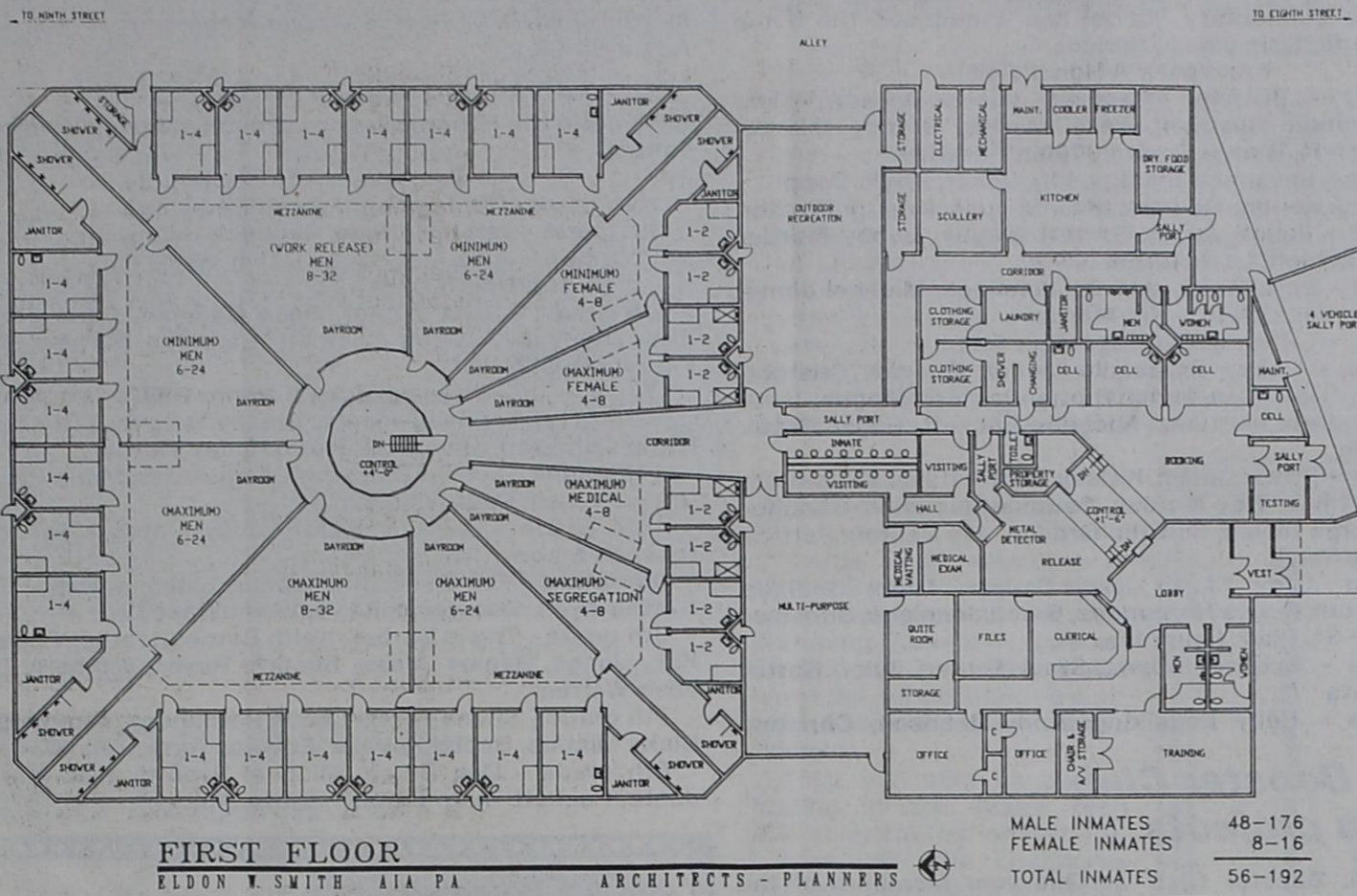
Plans for the new Curry County Jail
