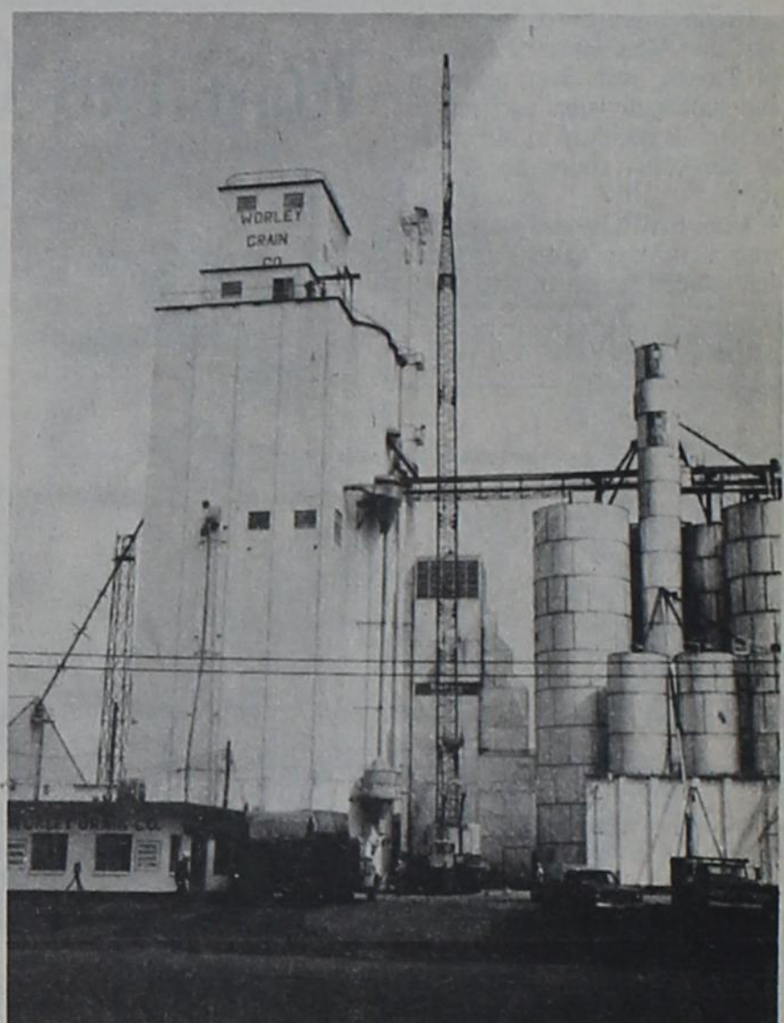
A REAL SKY HOOK - This 200-foot boom crane dominated the skyline this week in the Twin Cities. It was being used in the construction of an elevator leg in conjunction with Worley Grain's new grain dryer installation. The new dryer will have a 3,000 bushel per hour capacity and reduce grain moisture from 25 per cent to 18 per cent and later redry it to a storable 14 per cent moisture.
