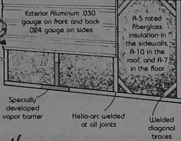
Cut-away Detailing Sidewall Construction
