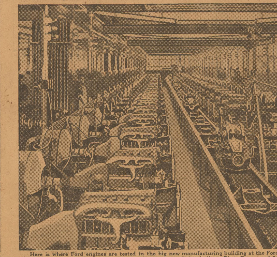
Here is where Ford engines are tested in the big new manufacturing building at the Ford Motor Company's River Rouge plant. All Ford engines are now being built at River Rouge and at the motor assembly line go immediately into the test department.
