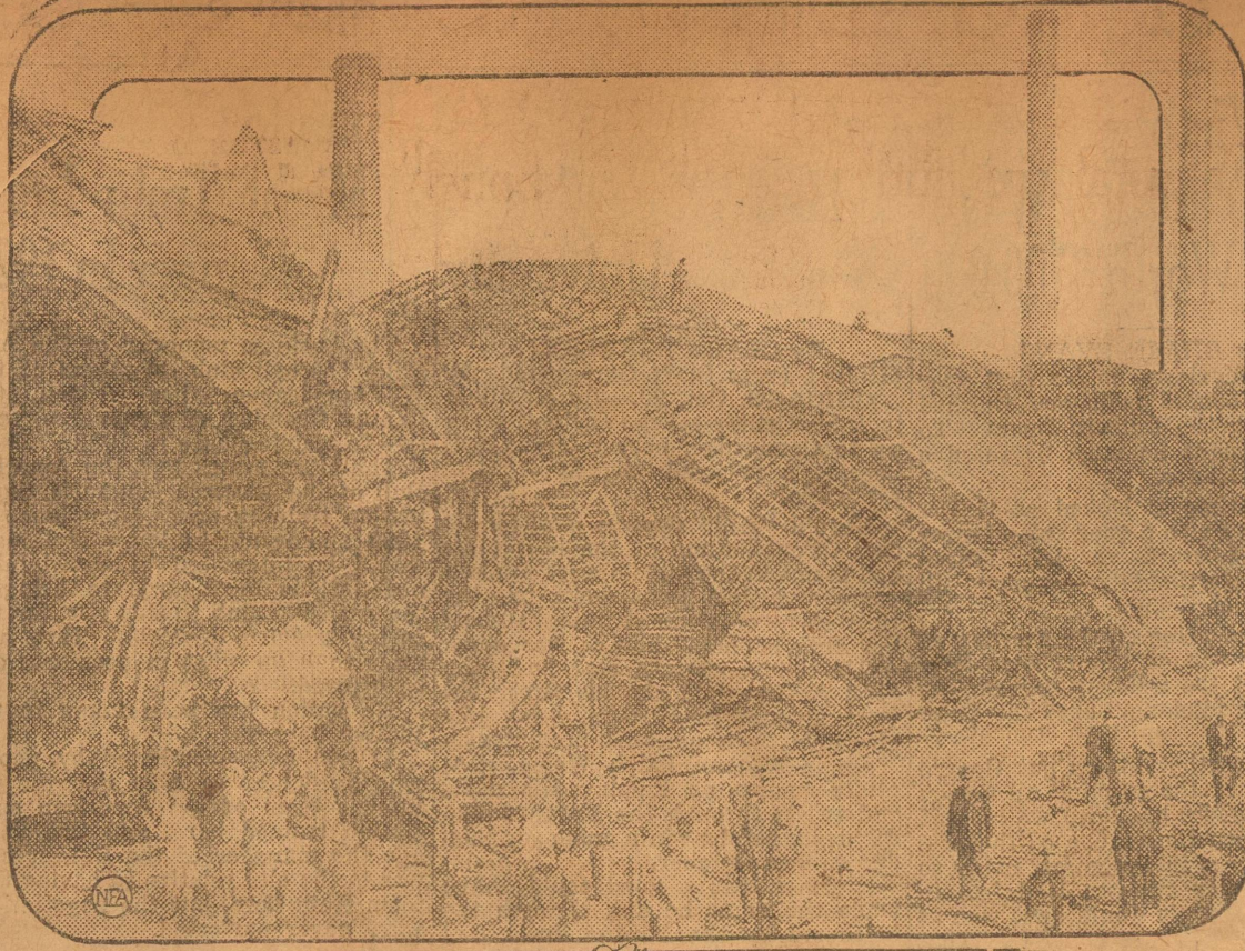
This picture indicates what happened when a concrete mixer, carried on a flatcar, protruding over the edge of a flatcar, caught on the steel supports of the union depot track shed at Peoria, Ill. Before the engineer knew what was happening the train had traveled the length of the building and it collapsed behind him. Though 89 trains a day use this terminal the accident happened when the place was practically empty and none was injured.
