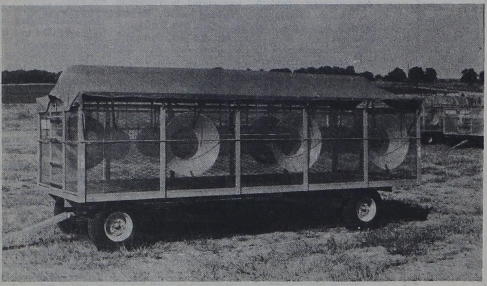
SOLAIR PEANUT DRYING NATURAL DRYING - A STEP TOWARD UPGRADING SOUTHWEST PEANUT QUALITY
