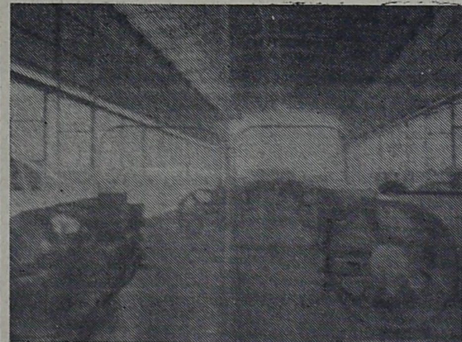
DRYING FACILITIES — This photo shows one drying facility which has 25 drying stalls. A heavy rail in the top of the shed carries a sampling machine which can sample any drying load at any time without having to transfer the peanuts to a sampler facility. This is a part of the Gorman Peanut Co. plant at Comyn.
