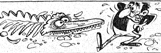
The earliest known fossils of living organisms on earth are about 3 billion years old.
